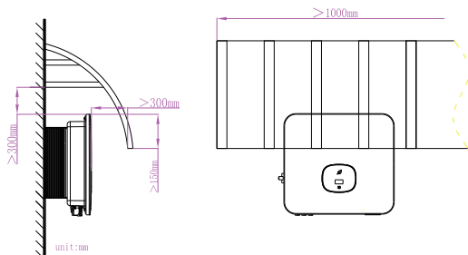
Fig 5.6 Parasole
