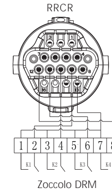
Fig 6.20 Collegamento inverter - RRCR
